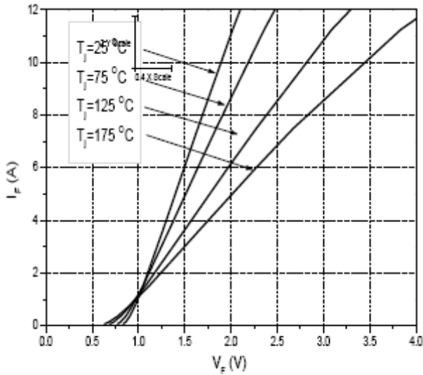
Figure 1. Forward Characteristics
